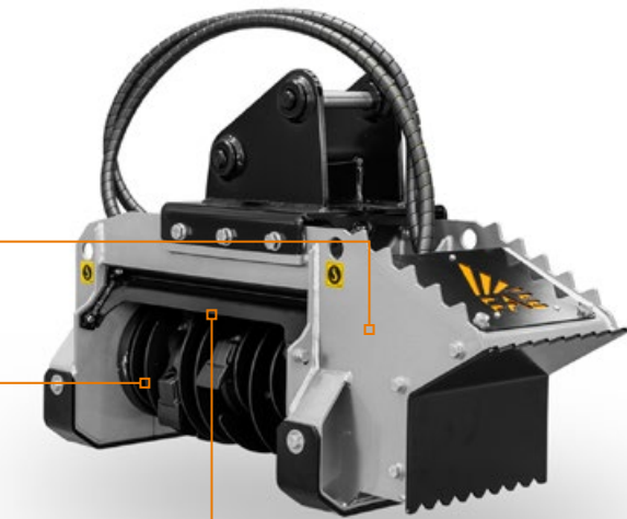
Fixed thumb bracket built into the frame useful for moving materials that need to be mulched
