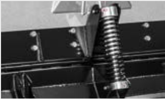
Dozing blade with springs system to level and compact the crushed material, creating a uniform base
